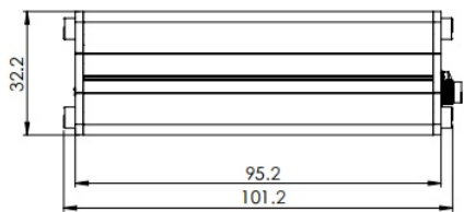
Right view
