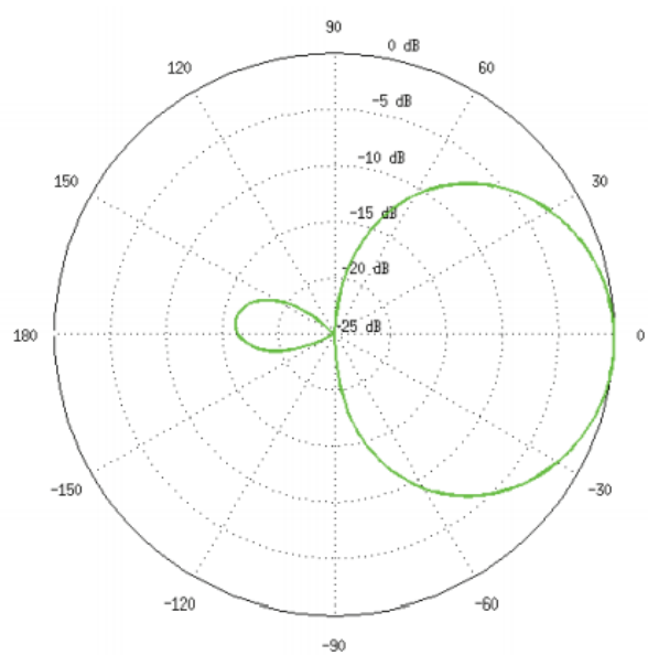
Horizontal Azimuth
