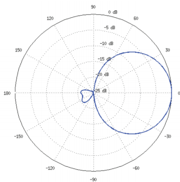
Horizontal Elevation
